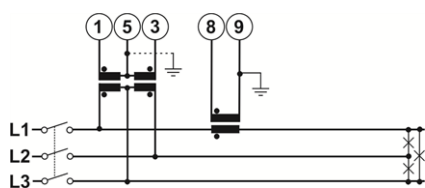
Fig. 14 AV6 balanced load
