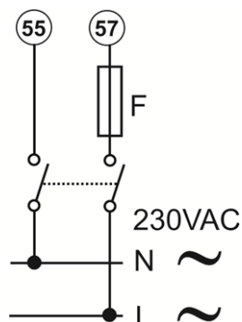
Fig. 22 D option. F = 250\text{ V}, 50\text{ mA}
