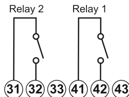
Fig. 27 Relay outputs
