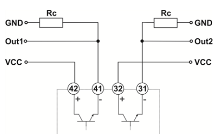
Fig. 26 Static outputs, VDC reference
